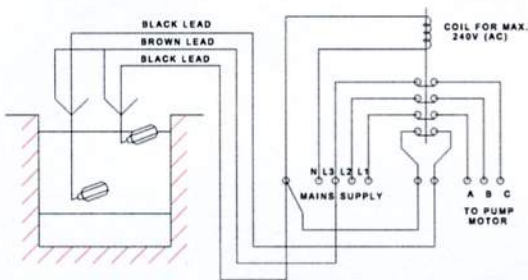
Connection diagram for automatically emptying tank
