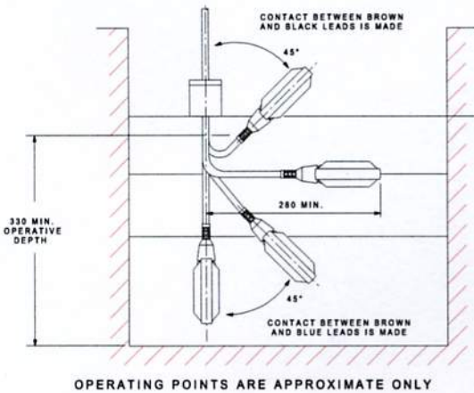
Connection diagram for automatically emptying tank
